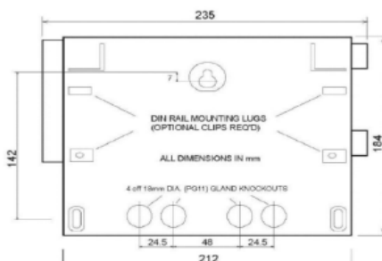
Sludge Finder 2 Drawing Back
